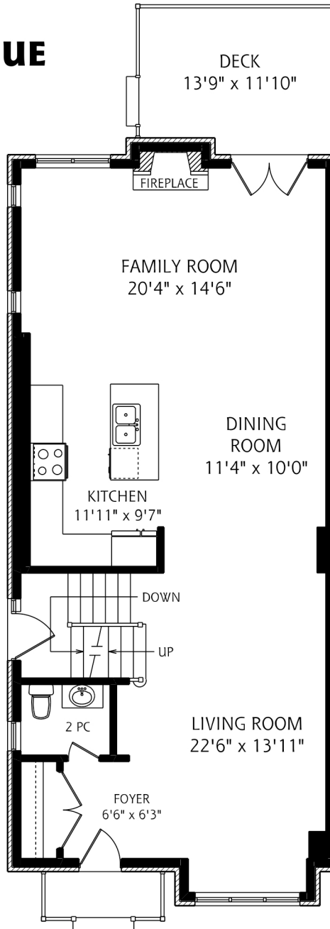
MAIN FLOOR 1,085 SQUARE FEET
